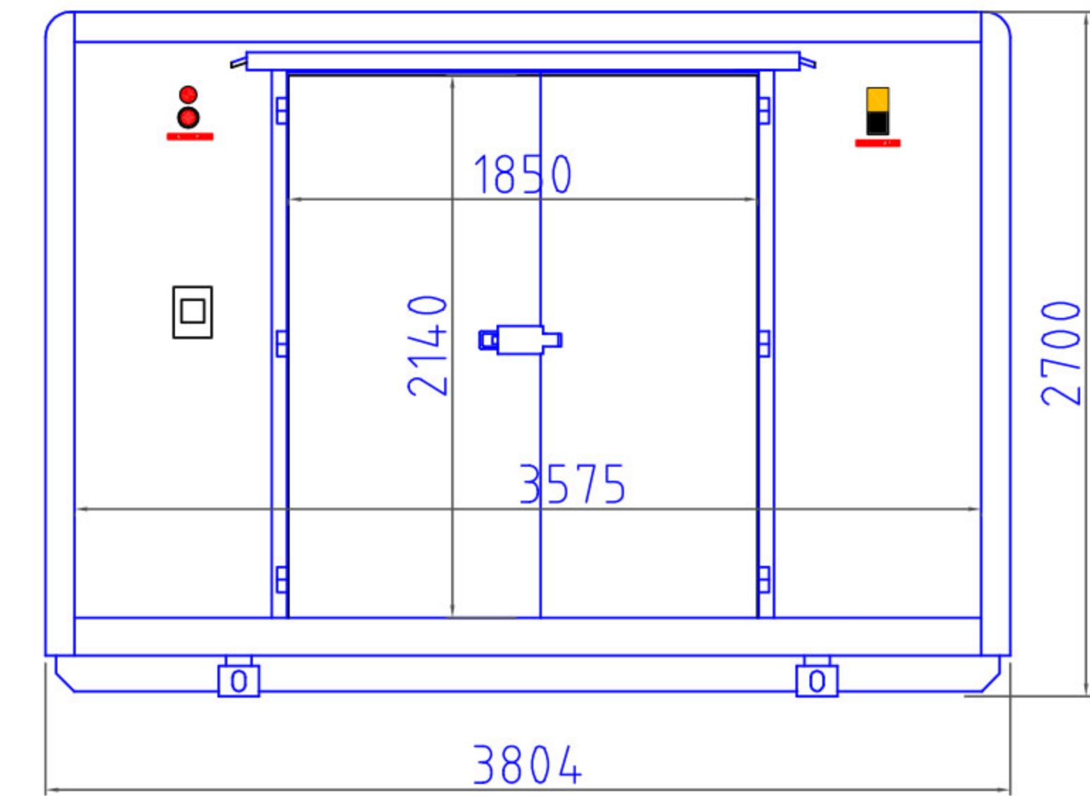
END VIEW
